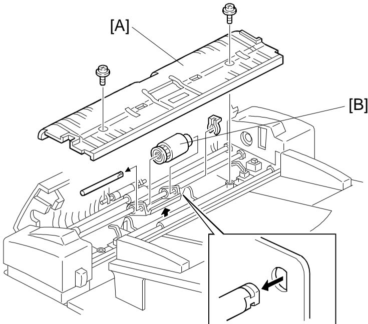
A: Upper Guide Plate (2 tapping screws), B: Separation Roller (1 clip)
